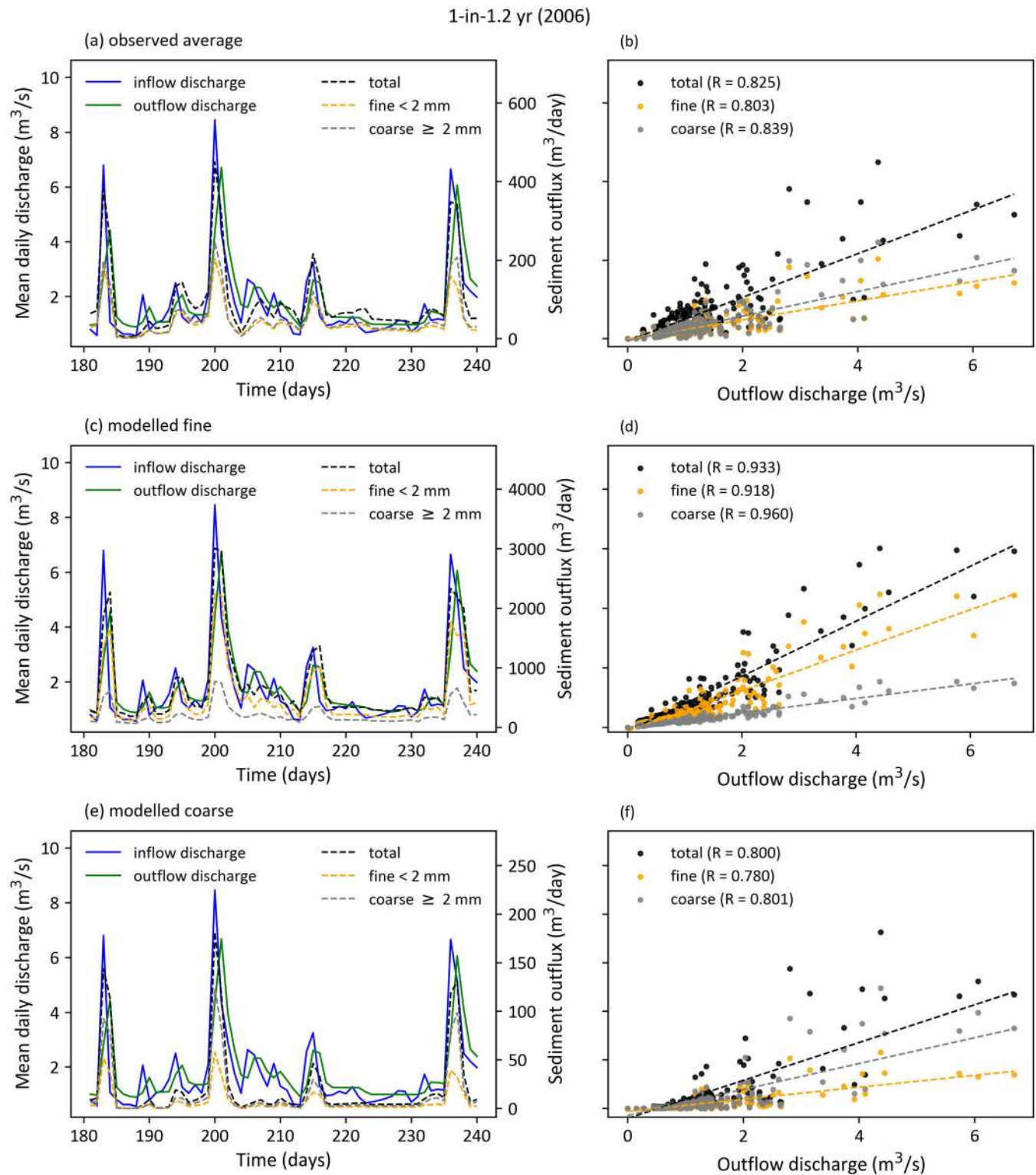
FIGURE 9 Computed water-sediment flows in the Nakkhu River. Left hand panels show inflow and outflow discharge hydrographs and daily sediment throughput time series for the Nakkhu River in 2006 (i.e., 1.2-year return period flood) for (a) observed GSD, (c) fine GSD and (e) coarse GSD. Right hand panels (b, d and f) show corresponding variations in sediment throughput with outflow river discharge for the three GSDs. The results display total, finer ( D < 2 mm) and coarser ( D \geq 2 mm) sediment throughputs obtained in pre-monsoon to post-monsoon periods during which the most significant changes were observed. [Color figure can be viewed at wileyonlinelibrary.com ]
