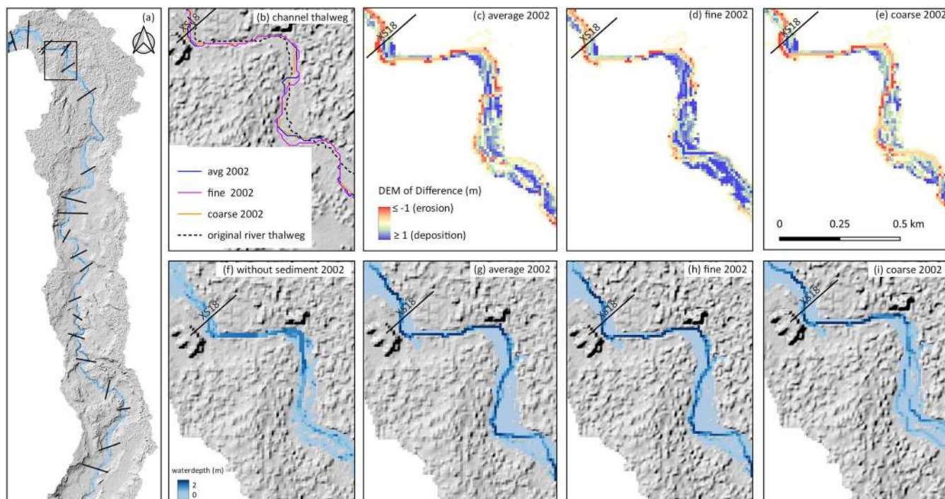
FIGURE 15 Morphological change along the Nakkhu River: (a) morphology change locations; (b) lateral channel migration; (c–e) erosion and deposition maps from DEM of difference; (f–i) flood extent maps in the downstream region near Location 18 [Color figure can be viewed at wileyonlinelibrary.com ]
