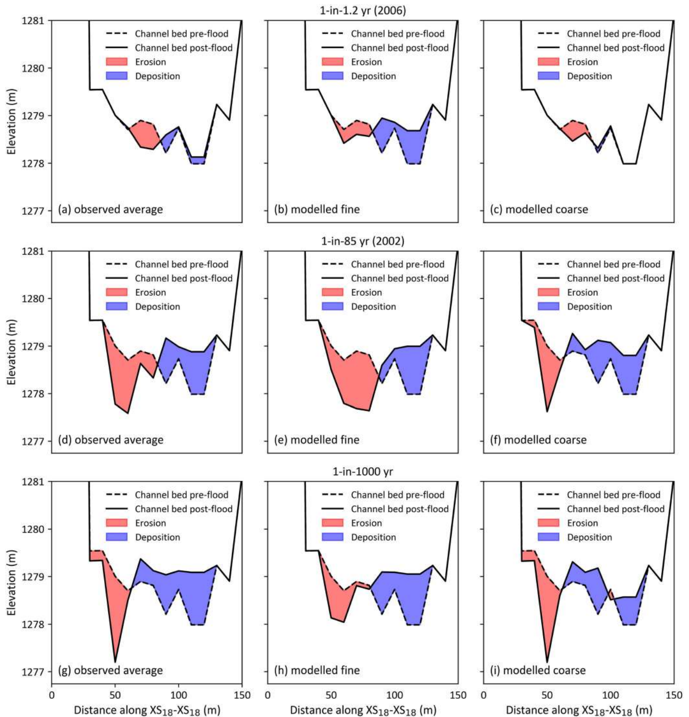
FIGURE 16 River cross-section profiles at Location 18 (shown in Figure 15) for average GSD (left column), fine GSD (middle column) and coarse GSD (right column) subject to 1.2-year (upper row), 85-year (middle row) and 1000-year (lower row) return period flood events. [Color figure can be viewed at wileyonlinelibrary.com ]
