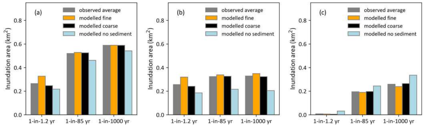
FIGURE 17 Histogram showing inundation areas after subtracting river channel obtained for 1.2-, 85- and 1000-year return period floods: (a) within the entire model domain regardless of water depth; (b) water depth \leq 0.5 m; and (c) water depth > 0.5 m. [Color figure can be viewed at wileyonlinelibrary.com ]
