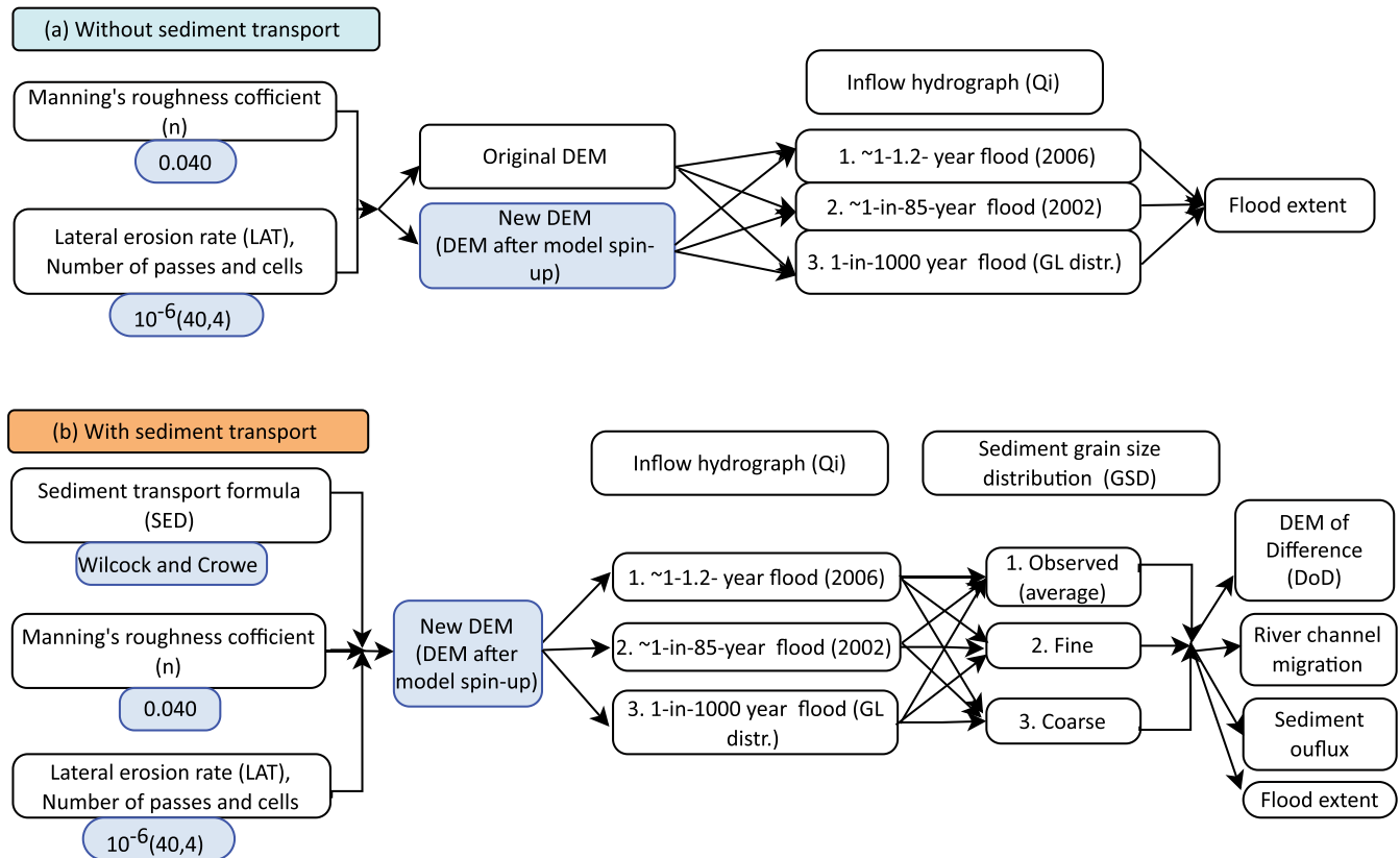
FIGURE 8 Flowchart highlighting key input parameters used for sensitivity analysis: (a) without and (b) with sediment transport. Blue-coloured boxes indicate model parameters that were found to give the best fit to observations of the Nakkhu River. [Color figure can be viewed at wileyonlinelibrary.com ]
