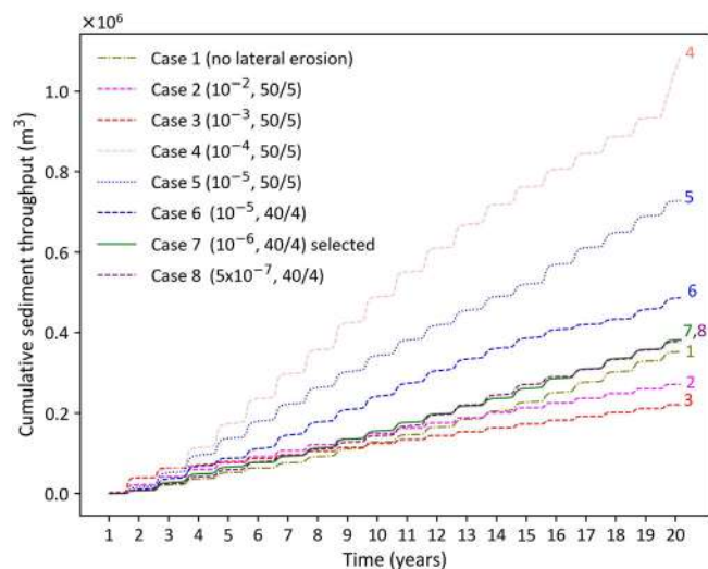
FIGURE 6 Cumulative sediment throughput over 20 years for different lateral erosion parameters. In the legend, the first value refers to the lateral erosion coefficient, and the fraction refers to the number of passes of the edge smoothing filter/the number of cells used to shift lateral erosion downstream. [Color figure can be viewed at wileyonlinelibrary.com ]
