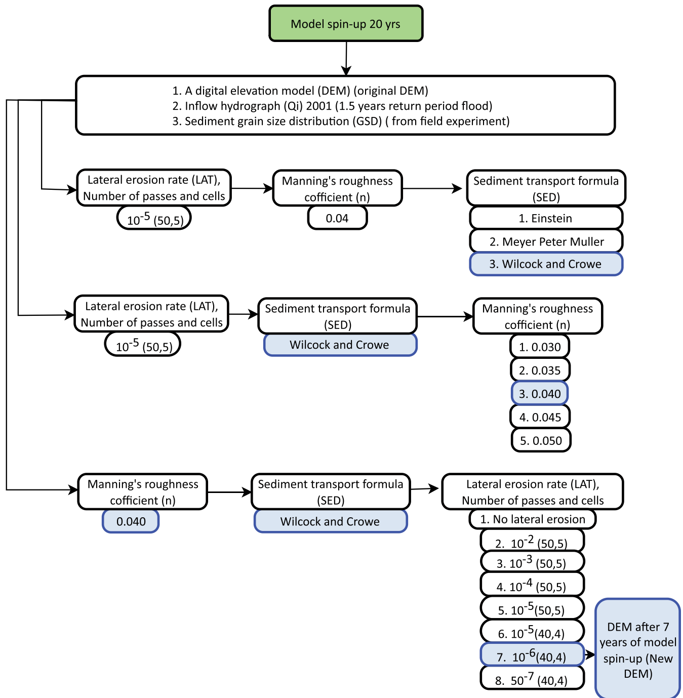
FIGURE 5 Flowchart highlighting key input parameters used for model spin-up. Blue-coloured boxes indicate model parameters that were found to give the best fit to observables in the Nakkhu River. [Color figure can be viewed at wileyonlinelibrary.com ]
