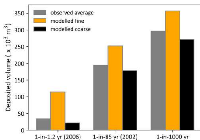
FIGURE 12 Deposited sediment volume obtained from DEM of Difference between pre-flood and post flood bed morphologies of the Nakkhu River reach for observed average, fine and coarse grain size distributions and 1.2-year return period flood (left), 85-year return period flood (middle) and 1000-year return period flood (right) [Color figure can be viewed at wileyonlinelibrary.com ]
