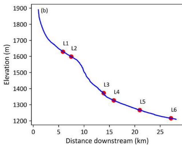
FIGURE 2 (a) Hillshade of the Nakkhu watershed with sediment sampling locations L1 to L6 marked along the river; (b) river profile with sampling locations indicated; and (c) scatter plot showing proportion of coarse ( D \geq 2 mm) sediment grain size distribution and median size ( D_{50} ) of collected samples at different locations after sieving. [Color figure can be viewed at wileyonlinelibrary.com ]
