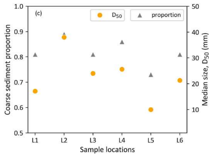
FIGURE 2 (a) Hillshade of the Nakkhu watershed with sediment sampling locations L1 to L6 marked along the river; (b) river profile with sampling locations indicated; and (c) scatter plot showing proportion of coarse ( D \geq 2 mm) sediment grain size distribution and median size ( D_{50} ) of collected samples at different locations after sieving. [Color figure can be viewed at wileyonlinelibrary.com ]
