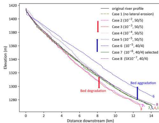
FIGURE 7 Original river bed profile and riverbed profiles obtained after model spin-up using different lateral erosion parameters. In the legend, the first value refers to the lateral erosion coefficient and the fraction refers to the number of passes of the edge smoothing filter/the number of cells used to shift lateral erosion downstream. [Color figure can be viewed at wileyonlinelibrary.com ]
