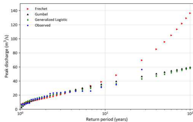
FIGURE 3 Gumbel, Fréchet and generalised logistic flow distributions fitted to the Nakkhu River from observed peak daily discharge data obtained at Khokana hydrological station, Nepal, from 1992 to 2017 inclusive. The Fréchet distribution tends to overestimate the observed data. [Color figure can be viewed at wileyonlinelibrary.com ]
