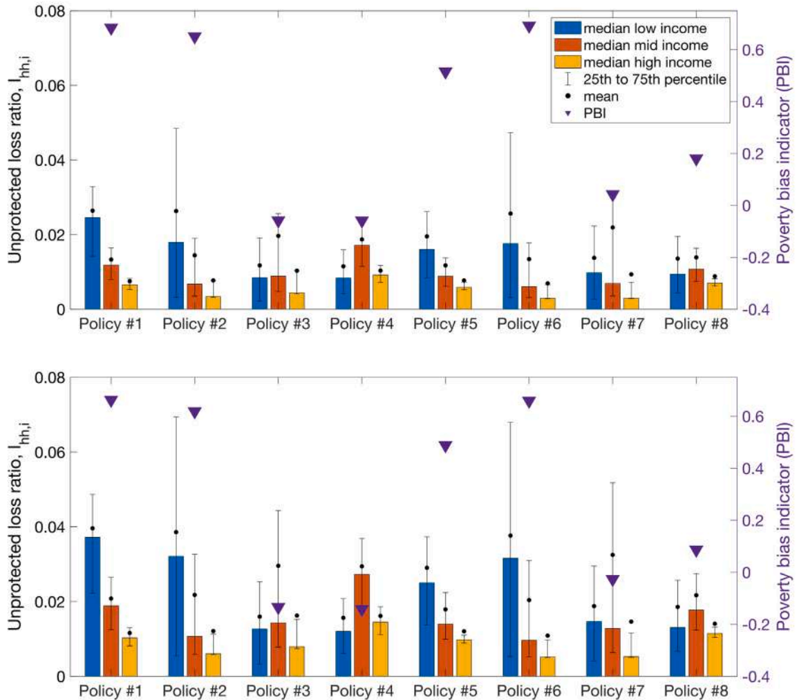
Fig. 10. I_{hh,i} calculated for candidate soft policies applied to TV50_total, considering two alternative assumptions about the time since the last characteristic event (in 50 years): 60 years (top panel) and 150 years (bottom panel). Corresponding PBI values are also shown.
