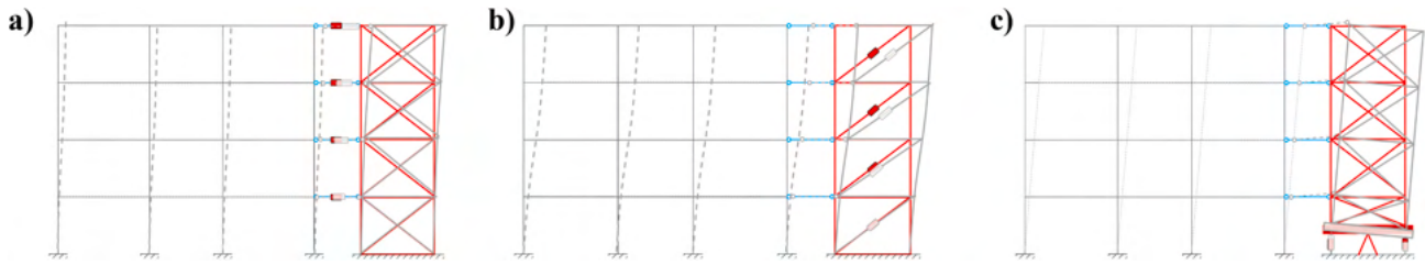
Fig. 13. Illustration of three categories of external dissipative systems: (a) dampers placed horizontally at the storey level between the frame and an external stiff contrasting structure; (b) dampers incorporated within a new shear deformable structure; (c) pinned rocking bracing with dampers located at the base.
