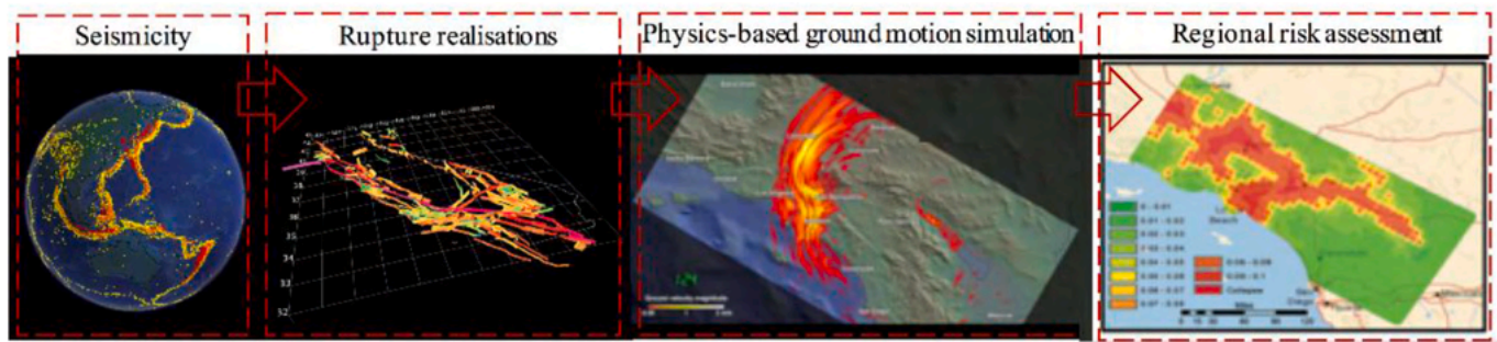
Fig. 2. Computational stages of the physics-based approach to modelling ground motions, from the tectonics and seismicity models to rupture realizations of potential events and the subsequent ground-motion simulations and risk assessments (adapted from Jones et al. [25] and the SCEC Community Fault Model 6 ).
